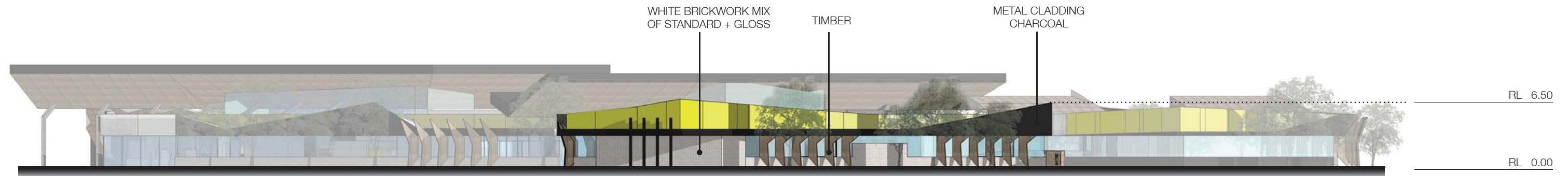
North Elevation
