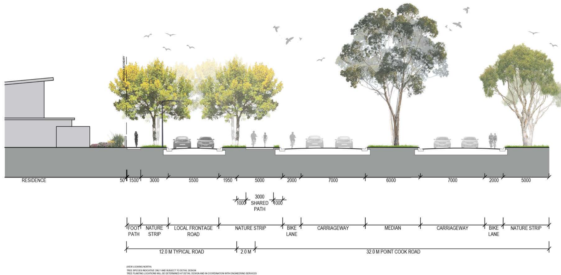
SECTION C - 12M LOCAL ACCESS STREET - 14M BUFFER TO POINT COOK ROAD CONDITION 1E 1:200@A3
