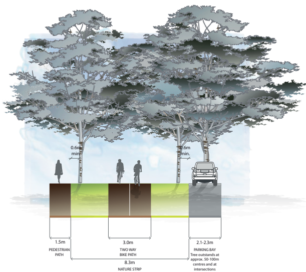
Cross Section Connector Street (25.5m) Two way off road bike path
