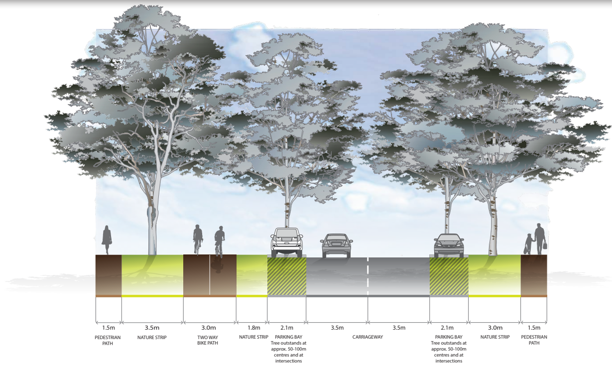
Cross Section Connector Street (25.5m) Two way off road bike path
