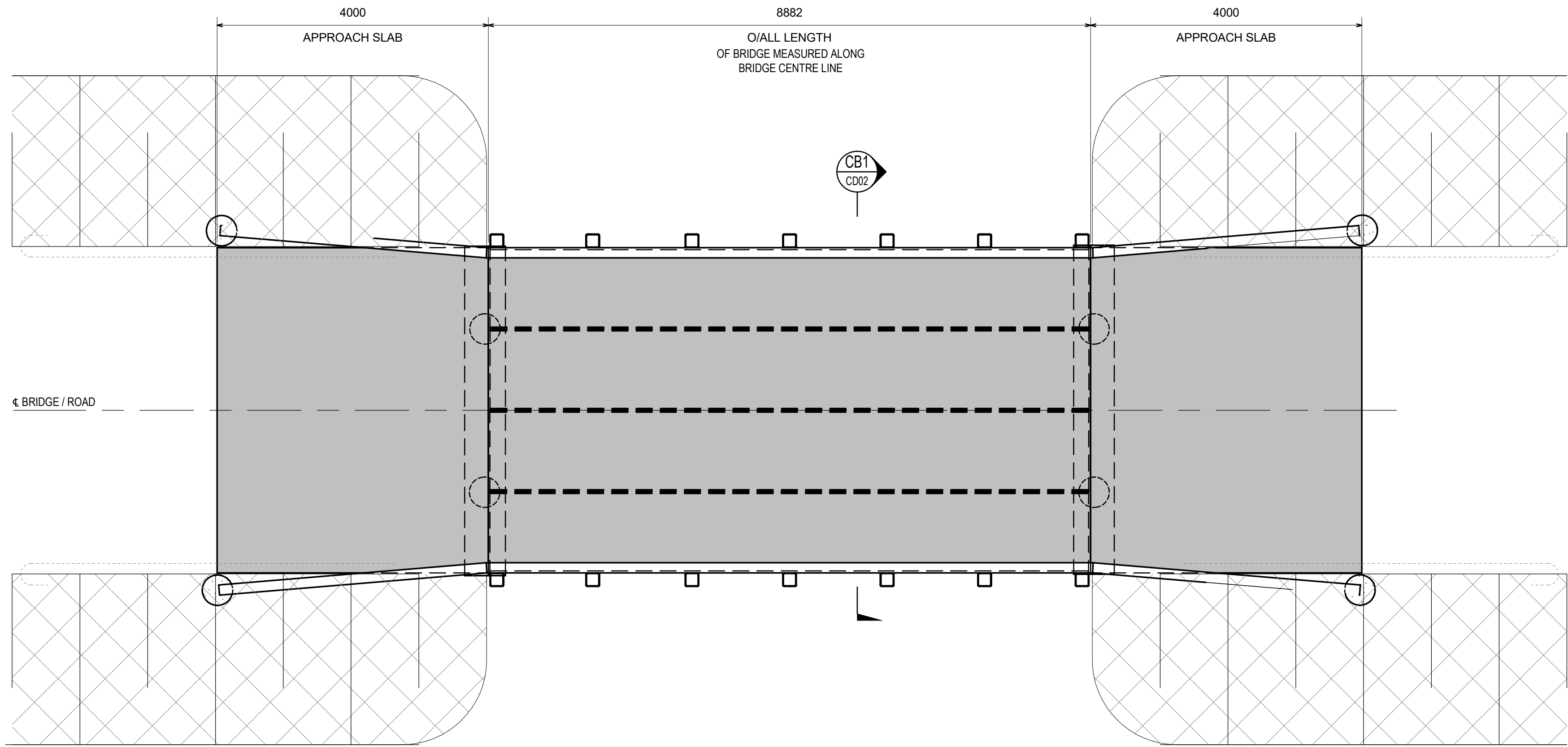
CU14 - GENERAL ARRANGEMENT - PLAN
