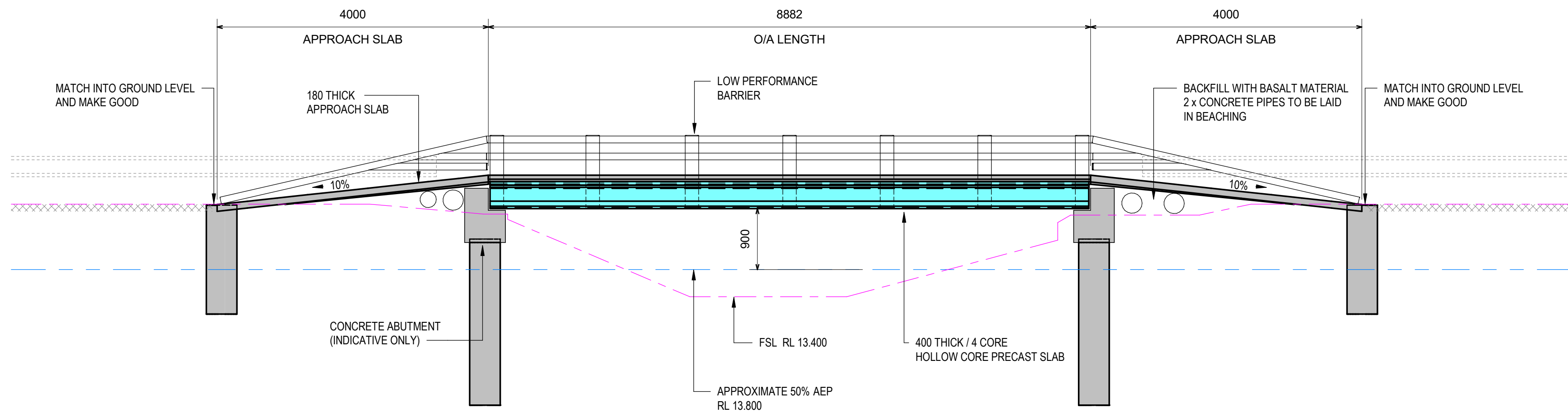
CU14 - ELEVATION
