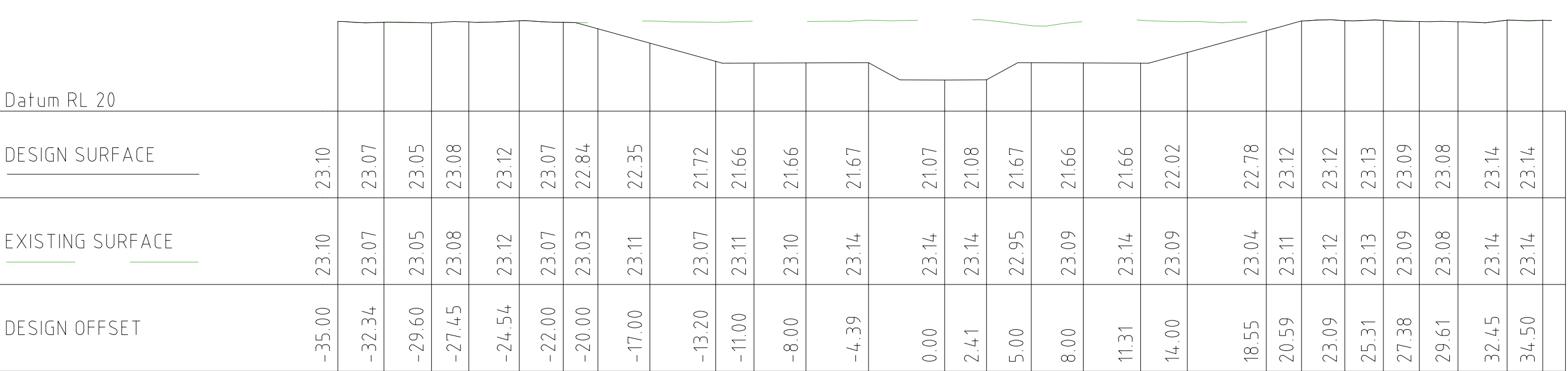
WEST WATERWAY CHAINAGE 2300 1:250 (H) 1:125 (V) 2300046
