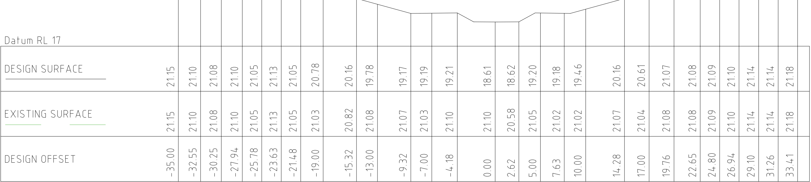
WEST WATERWAY CHAINAGE 1600 1:250 (H) 1:125 (V) 1600045
