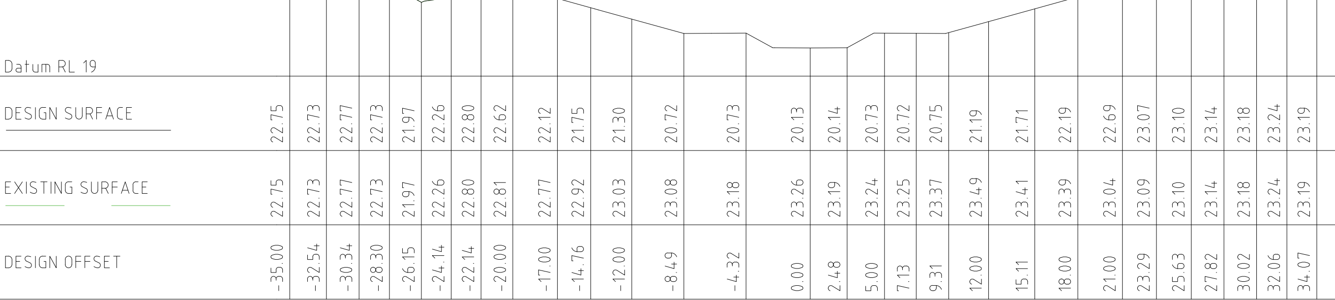
WEST WATERWAY CHAINAGE 2000 1:250 (H) 1:125 (V) 2000045
