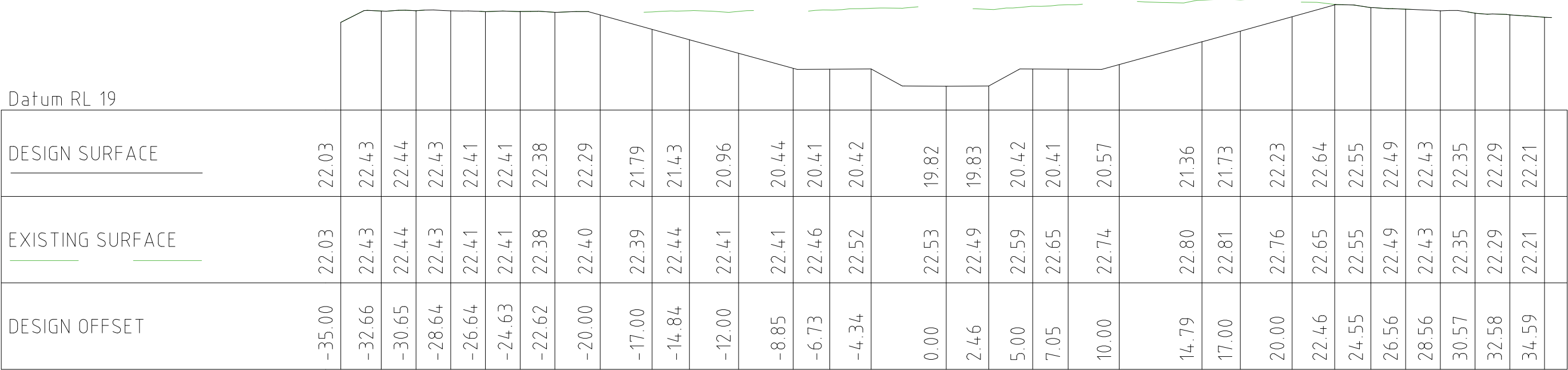
WEST WATERWAY CHAINAGE 1900 1:250 (H) 1:125 (V) 1800045
