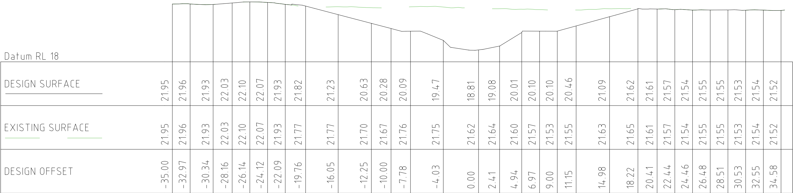
WEST WATERWAY CHAINAGE 1800 1:250 (H) 1:125 (V) 1800045
