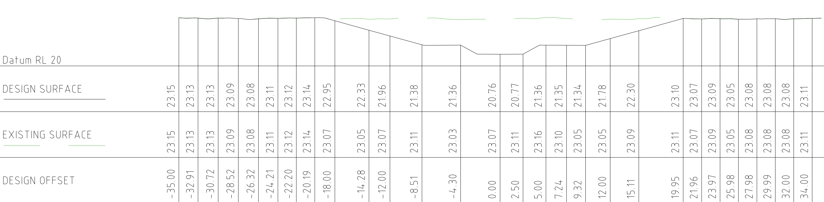
WEST WATERWAY CHAINAGE 2200 1:250 (H) 1:125 (V) 2200046
