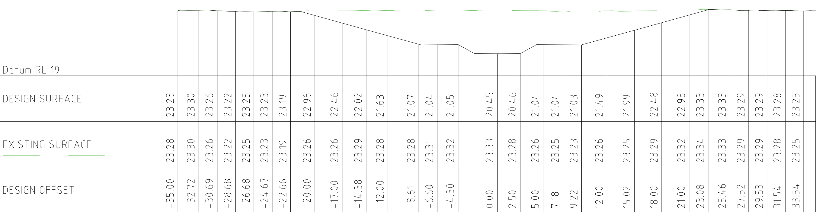
WEST WATERWAY CHAINAGE 2100 1:250 (H) 1:125 (V) 2100045
